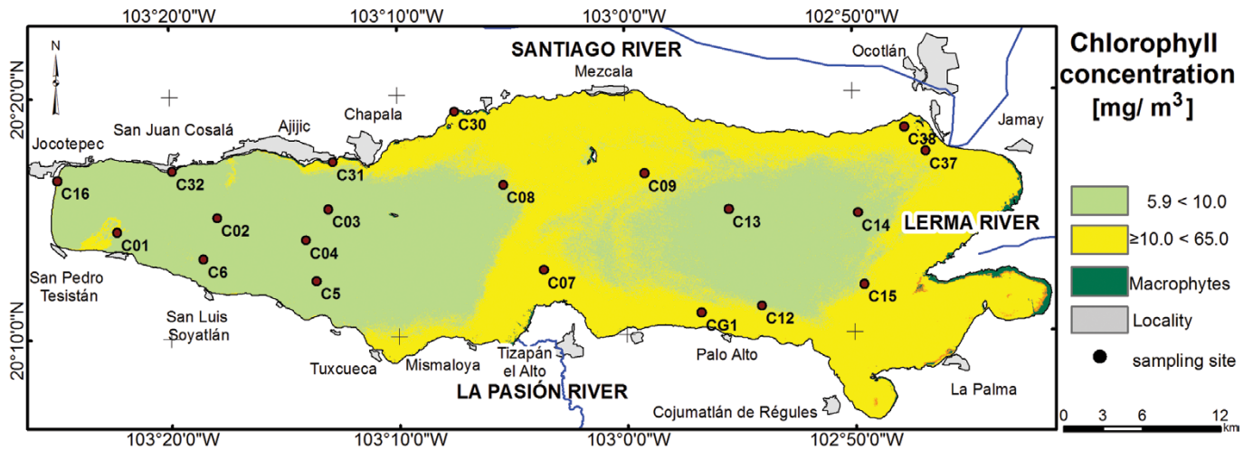
Figure 2. The Chl- a concentration (mg/m 3 ), calculated from the SPOT B3/B2 ratio to enhance the spectral response of Chl- a , was only determined in areas where macrophytes (water hyacinth and cattails) were not present, as recorded from the ground truthing work. Those areas are labeled as class-macrophytes.
