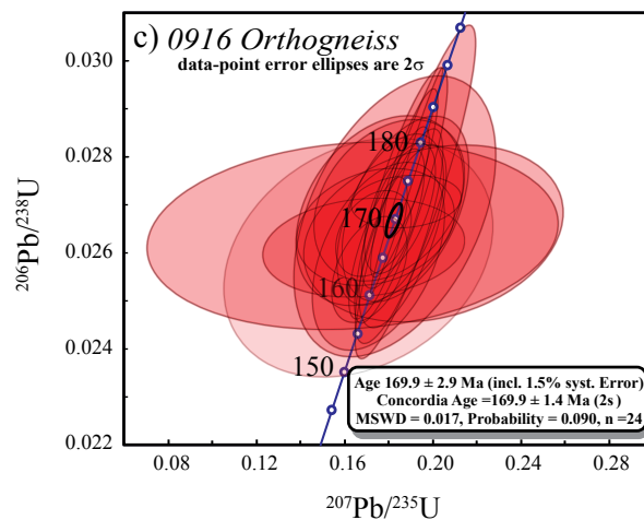
Figure 12. a) and b) Cathodoluminescence images and ^{206}\text{Pb}^*/^{238}\text{U} ages for selected laser spots on individual zircon grains from banded gneiss 0916. c) U-Pb concordia diagram showing U-Pb isotope data of zircons from sample 0916. Error ellipses of individual spots are 2\sigma .
