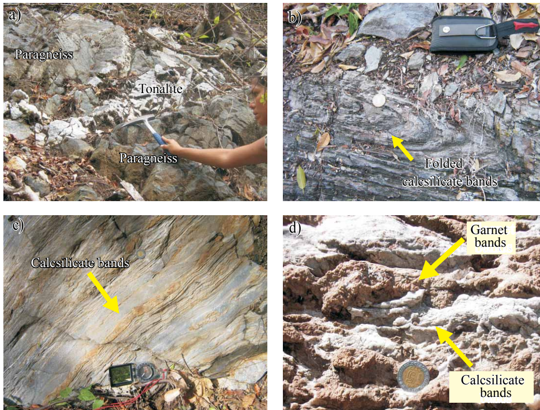
Figure 4. Metasedimentary rocks exposed in the Papelillo canyon. a) Garnet-bearing paragneiss in contact with a tonalitic body. b) Folded calcsilicates affected by contact metamorphism. c) Folded and banded calcsilicate rocks. d) Calcsilicate rocks with garnet bands.
