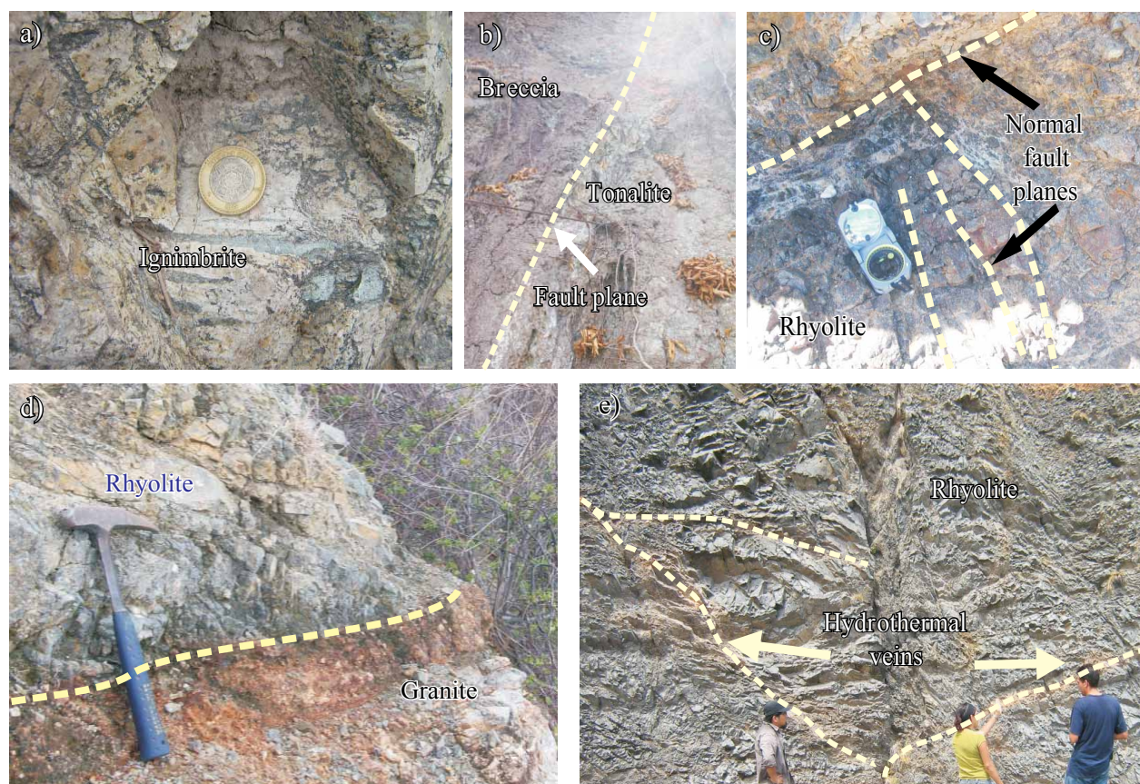
Figure 6. Volcanic rocks. a) Massive and altered ignimbrite unit exposed in the northwestern part of the island. b) Normal fault plane that separates tonalites from a massive volcanic breccia in the Papelillo canyon. c) Faulted and fractured rhyolite near Laguna del Toro. d) Rhyolite discordantly covering granitic rocks near Camarón. e) Faulted and fractured rhyolite with hydrothermal veins near Camarón.
